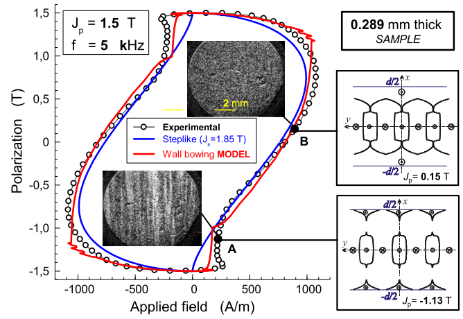
Fig. 12. Experimental cycle taken between \pm 1.5 T at 5 kHz on a 0.289 mm thick HGO sheet (symbols) and cycle predicted by the dw bowing numerical model. The dw patterns theoretically envisaged to occur at two different times A and B along the semi-cycle (right-hand side) are compared with the correspondingly obtained surface magneto-optical images. The appearance of a horizontal front is contemplated by the calculations. The hysteresis loop predicted for the ideal case of step-like constitutive magnetization curve is also shown.
