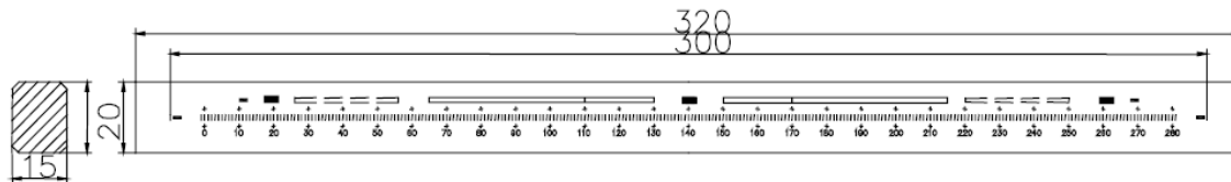
Main graduation : 280 mm length, 1 mm pitch, CD 4 μm, 1 mm line length
