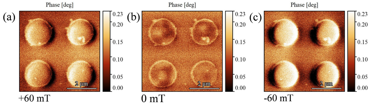
Fig. 4. Magnetic domain textures of \text{Fe}_{70}\text{Ga}_{30} disks with diameter of 1.8\ \mu\text{m} with in-plane applied field of +60\ \text{mT} (positive saturation), 0\ \text{mT} (remanence) and -60\ \text{mT} (negative saturation) is shown by (a), (b) and (c), respectively.
