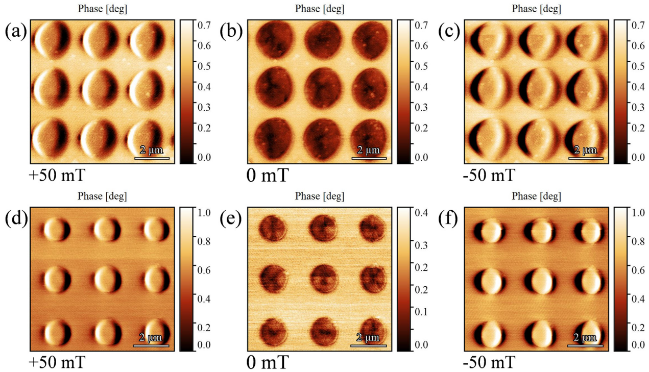
Fig. 2. Magnetic domain textures of the \text{Fe}_{80}\text{Ga}_{20} disks of diameter 2.3\ \mu\text{m} and 1.4\ \mu\text{m} measured using MFM. (a), (b) and (c) represents the 2.3\ \mu\text{m} disks with in-plane magnetic field of +50\ \text{mT} (positive saturation), 0\ \text{mT} (remanence) and -50\ \text{mT} (negative saturation), respectively. (d), (e) and (f) represents the 1.4\ \mu\text{m} disks at +50\ \text{mT} , 0\ \text{mT} and -50\ \text{mT} , respectively.
