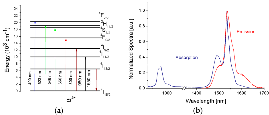
Figure 3. (a) Typical energy level diagram of Er^{3+} ions in phosphate glasses; (b) Common absorption and emission spectra of Er^{3+} ions in phosphate glasses (adapted from [12]).
