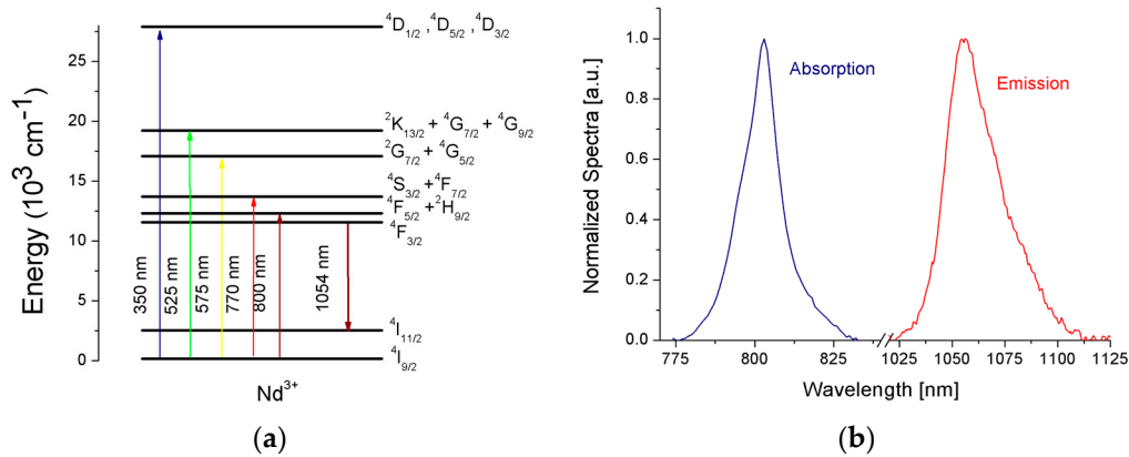
Figure 2. (a) Typical energy level diagram of Nd^{3+} ions in phosphate glasses; (b) Typical absorption and emission spectra of Nd^{3+} ions in phosphate glasses (adapted from [27]).
