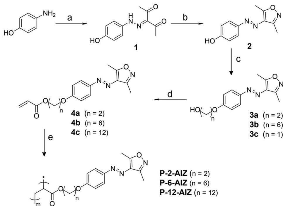
Figure 2. Synthesis of polymers containing AIZs. Reagent and conditions: a) \text{NaNO}_2 , 0 °C, 1 h, 2,4-pentanedione, \text{NaOAc} , \text{H}_2\text{O} , rt, 18 h, b) \text{NH}_2\text{OH} \text{HCl} , \text{Na}_2\text{CO}_3 , \text{EtOH} , reflux, 18 h c) 2-bromo-1-ethanol (for 3a) or 6-chloro-1-hexanol (for 3b) or 12-bromo-dodecanol (for 3c), \text{K}_2\text{CO}_3 , \text{KI} , \text{DMF} , 80 °C; 18 h, d) acryloyl chloride, \text{TEA} , \text{CH}_2\text{Cl}_2 , rt; 2 h e) \text{AIBN} , toluene, 80 °C; 24 h.
