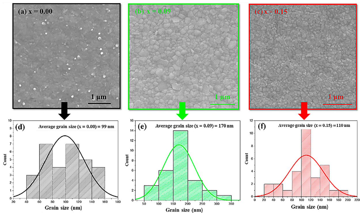
Figure 6. Top view SEM images of the perovskite films at different CsBr-doping concentrations: (a) x = 0.00 , (b) x = 0.09 , and (c) x = 0.15 ; (d–f) grain size distribution of the perovskite films at different CsBr-doping concentrations.
