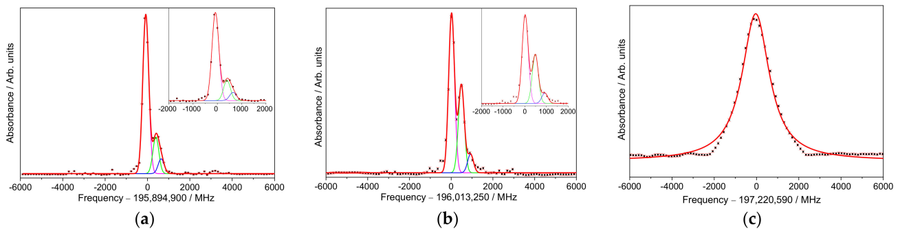
Figure 5. \text{Er}^{3+} absorption spectra and their fitting of sample \text{Er}:\text{LiYF}_4 35 ppm for (a) {}^4\text{I}_{15/2} \Gamma_{56}^{(1)} \rightarrow {}^4\text{I}_{13/2} \Gamma_{78}^{(1)} ; (b) {}^4\text{I}_{15/2} \Gamma_{56}^{(1)} \rightarrow {}^4\text{I}_{13/2} \Gamma_{56}^{(1)} ; (c) {}^4\text{I}_{15/2} \Gamma_{56}^{(1)} \rightarrow {}^4\text{I}_{13/2} \Gamma_{78}^{(2)} . The red line is the total nonlinear fitting, the magenta, green, and blue lines are the individual peaks that contribute to the convolution.
