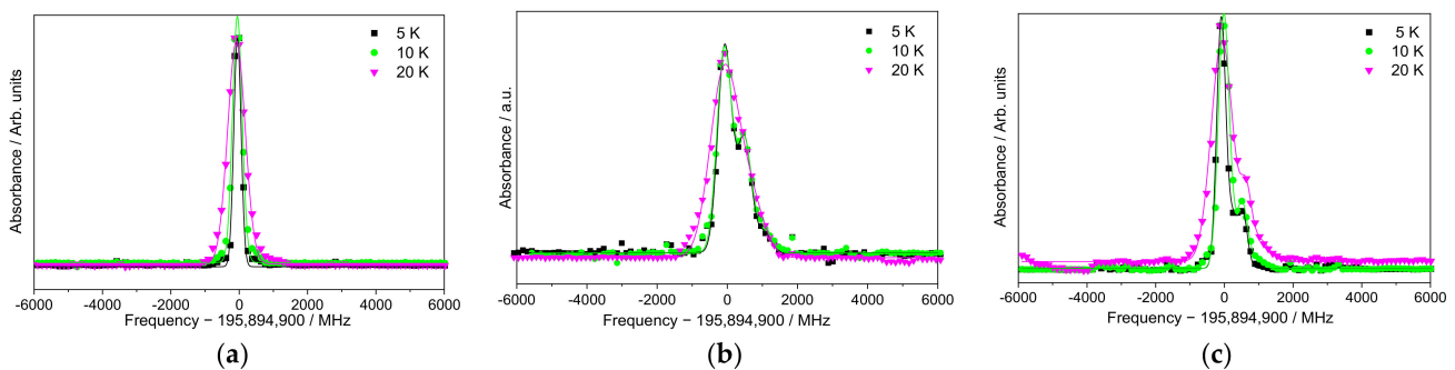
Figure 6. \text{Er}^{3+} absorption spectra for transition {}^4\text{I}_{15/2} \Gamma_{56}^{(1)} \rightarrow {}^4\text{I}_{13/2} \Gamma_{78}^{(1)} at 5, 10, and 20 K for samples (a) {}^{166}\text{Er}:\text{LiYF}_4 100 ppm; (b) \text{Er}:\text{LiYF}_4 100 ppm; (c) \text{Er}:\text{LiYF}_4 35 ppm.
