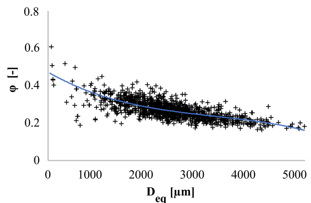
Figure 7. Sphericity vs. void equivalent diameter and polynomial trendline ( n=3 ; R^2 = 0.51 ).
