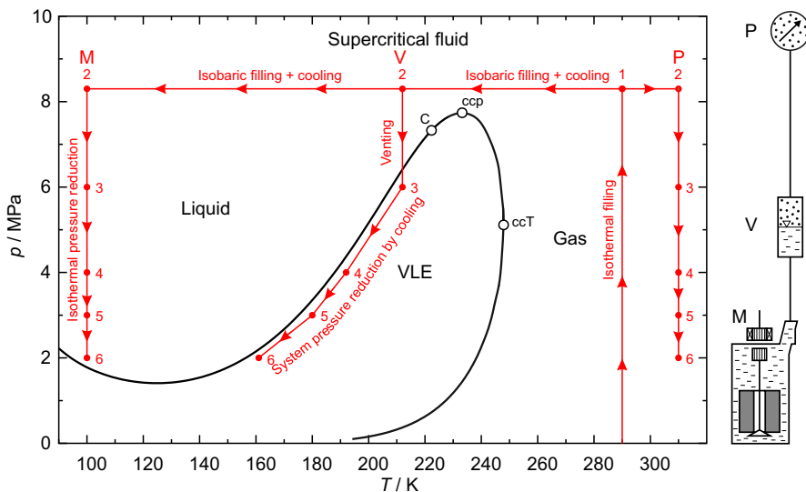
Fig. 1 Left: Principle of the filling and liquefaction procedure shown in a p , T -diagram for a methane-rich gas mixture containing hydrogen. As an example, the points to be measured at T = 100 K are plotted. For illustration purposes, a composition was chosen that differs from the mixtures investigated in this work (compare with Fig. S3 in the Online Resource 1). The phase envelope was calculated using the GERG-2008 equation of state of Kunz and Wagner [7, 8]. Right: Schematic presentation of the measurement system consisting of the measuring cell (M), VLE-cell (V) and pressure measurement system (P)
