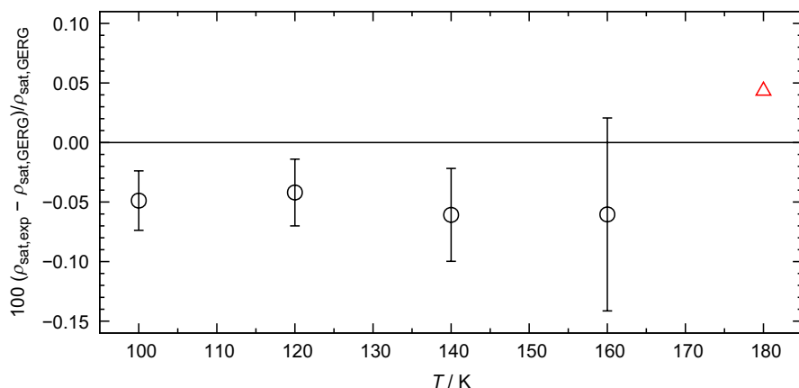
Fig. 3 Relative deviations of experimental saturated-liquid densities \rho_{\text{sat,exp}} for two biomethane-like mixtures from densities \rho_{\text{sat,GERG}} calculated with the GERG-2008 equation of state [7, 8] (zero line). ( p_{\text{sat}} , \rho_{\text{sat}} , T , x ) data of the present work: LBG I: \circ ; BG II: \triangle . The uncertainties of our new saturated-liquid density data are illustrated with error bars (also see Table 5). For the LBG II mixture, no error bars are plotted since they are outside the scaling of the ordinate. The compositions of the LBG mixtures are given in Table 1
