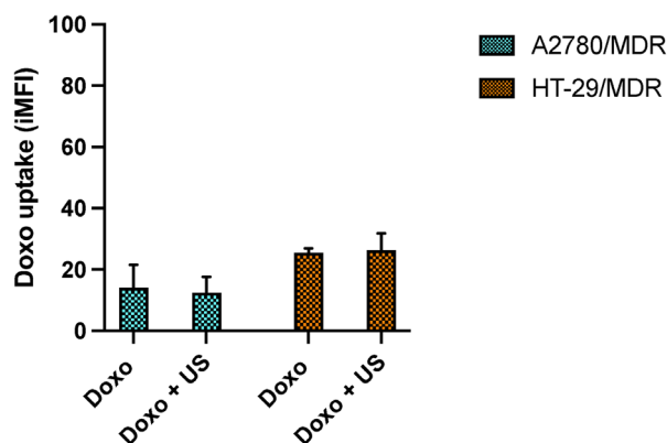
Figure 6. Doxo cellular uptake in MDR cell lines before and just after US exposure. A2780/MDR and HT-29/MDR cells were exposed to Doxo 0.5 and 1.0 \mu M for 1 h, respectively, and subsequently exposed to US (0.63 W cm -2 , 1.505 MHz, 3 min, 70% DC). Results are expressed as integrated mean of fluorescence intensity (iMFI).
