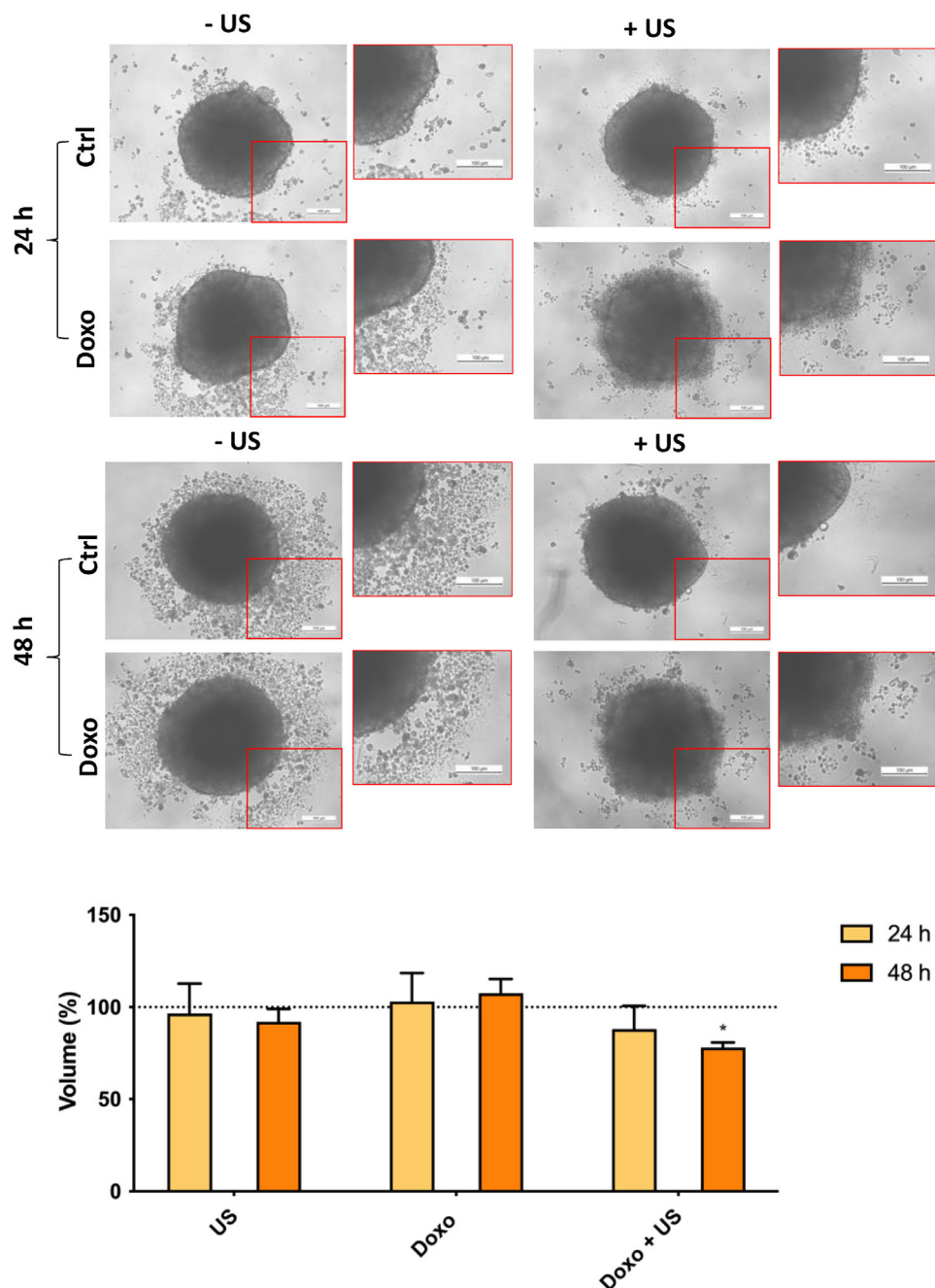
Figure 12. Effect of the US exposure of Doxo-pre-incubated HT-29/MDR spheroids. Spheroids were incubated with Doxo (20 \mu M) for 1 h and then exposed to US (1.66 W cm -2 , 1.505 MHz, 5 min, 70% DC). In the upper part of the figure, representative spheroids' images have been reported (magnification: 10x; scale bars: 100 \mu m) along with a 25% enlargement of the highlighted red quadrant. In the lower part of the figure, spheroids' volumes have been reported after 24 and 48 h from US exposure and results are expressed as volume percentage of treated spheroids versus untreated spheroids (the volume of untreated spheroids is represented by the dashed line). Statistical significance versus untreated spheroids (Ctrl): * p \leq 0.05 .
