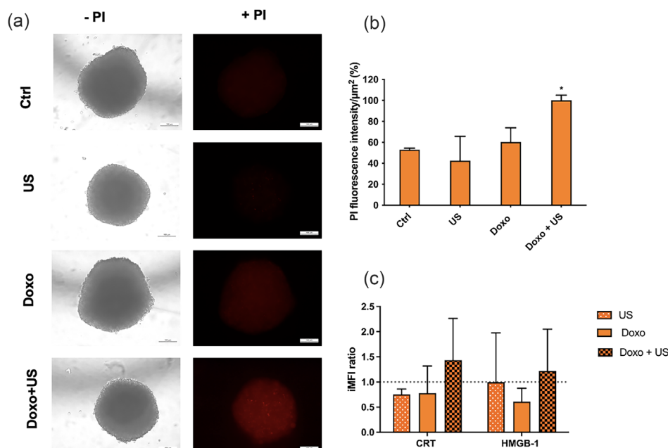
Figure 13. Evaluation of cell death and occurrence of CRT and HMGB-1 after SDT on HT-29/MDR spheroids. Spheroids were incubated with Doxo (20 μM) for 1 h and then exposed to US (1.66 W cm -2 , 1.505 MHz, 5 min, 70% DC). A) After 48 h, spheroids were stained with PI (100 μg mL -1 ) (magnification: 10x; scale bars: 100 μm). B) PI fluorescence quantification as mean of percentage of PI intensity μm -2 ± SD. Statistically significant difference of treated spheroids versus untreated spheroids (Ctrl): * p ≤ 0.05. C) CRT and HMGB-1 occurrence was detected at 6 and 48 h after the treatment, respectively, and results were expressed as iMFI ratio (CRT and HMGB-1 level in untreated cells is represented by the dashed line).
