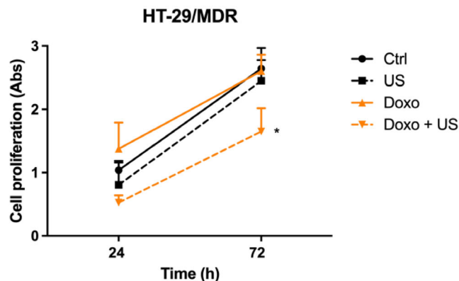
Figure 5. Effect on cell proliferation of the US exposure of Doxo-pre-incubated A2780/MDR and HT-29/MDR cells. A2780/MDR and HT-29/MDR cells were incubated for 1 h with Doxo 0.5 and 1.0 \mu M, respectively, and subsequently exposed to US (0.63 W cm -2 , 1.505 MHz, 3 min, 70% DC). Cell proliferation was assessed by using WST-1 assay after 24 and 72 h. Statistical significance versus untreated cells (Ctrl): * p \leq 0.05 , ** p \leq 0.01 .
