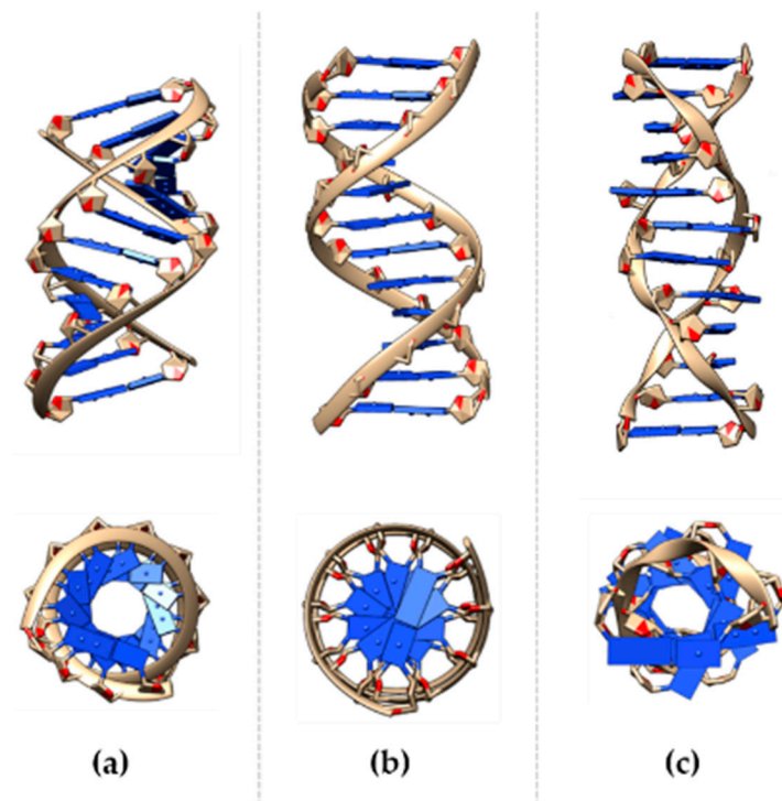
Figure 1. DNA helix in the (a) A-, (b) B-, and (c) Z-form lateral and upper view. A- and B-DNA structures were built and viewed using the program Chimera [3] for the arbitrary sequence ATCGATCGATCG; Z-form refers to the dodecamer TCGCGCGCGCGCG [4].
